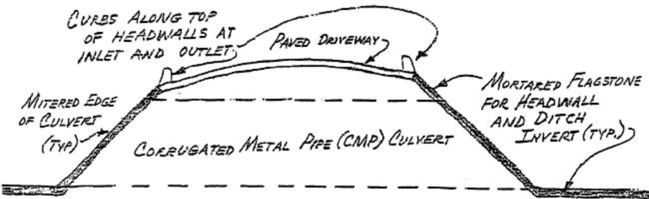
DRIVEWAY CULVERT PROFILE (NOT TO SCALE)
