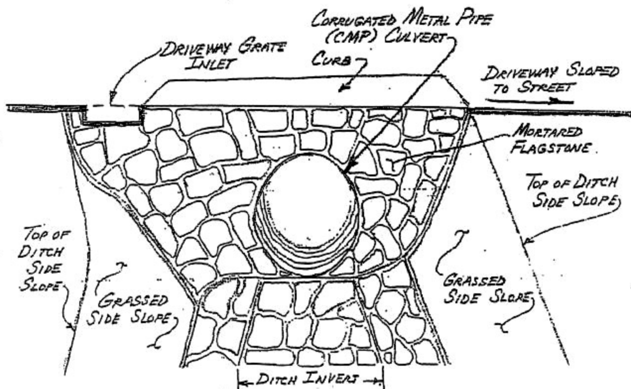
DRIVEWAY CULVERT HEADWALL (NOT TO SCALE)
